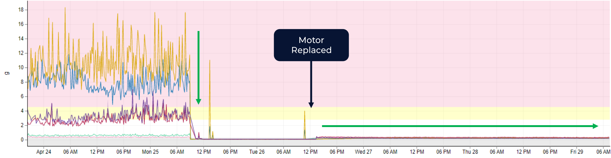
Stage 2 Bearing Fault Vibration Pattern
